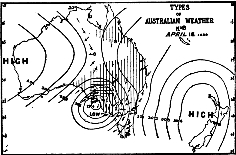
Cyclone in high latitudes from Monsoonal depression 8 to 10
